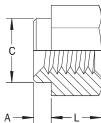
Thread sizes 0-80, S1, S1.2, S1.4 and M1.6
